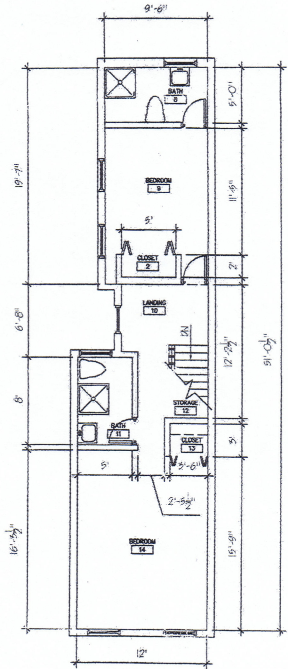
517 SECOND FLOOR PLAN 1/8" = 1'-0"
