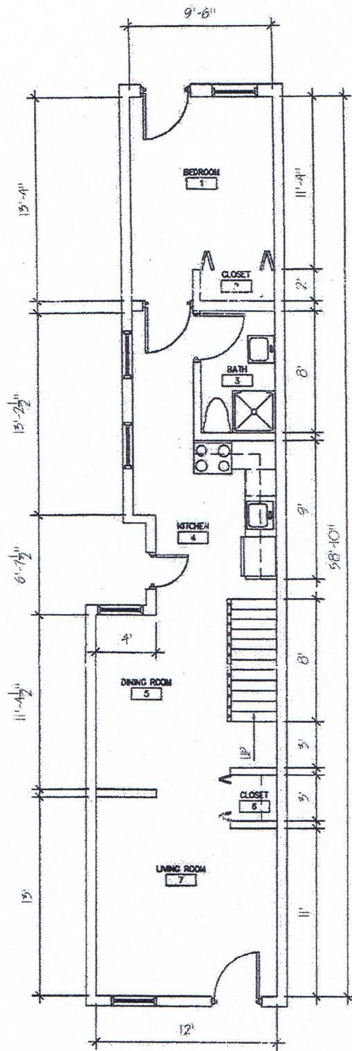
517 FIRST FLOOR PLAN 1/8" = 1'-0"
